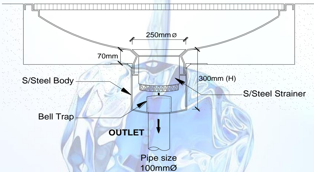
SECTION VIEW
