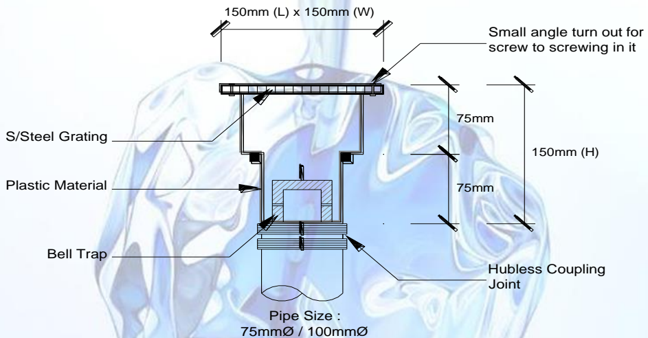
SECTION VIEW
