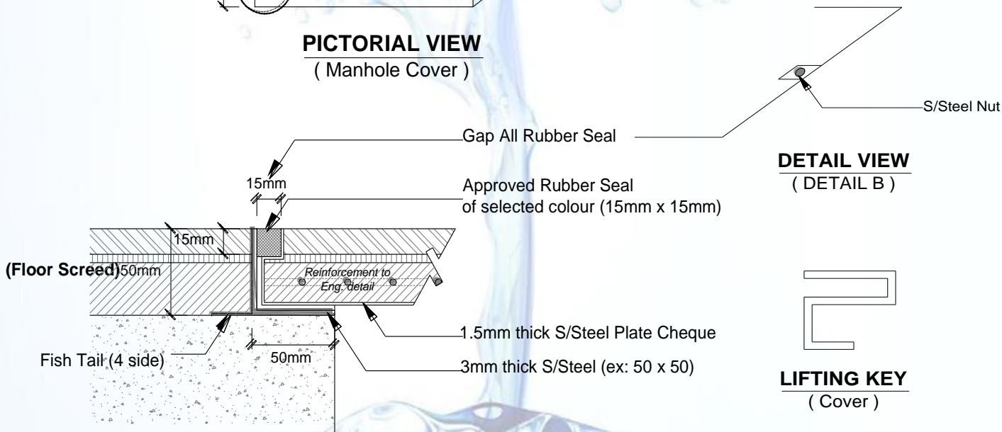
DETAIL VIEW ( DETAIL A )
