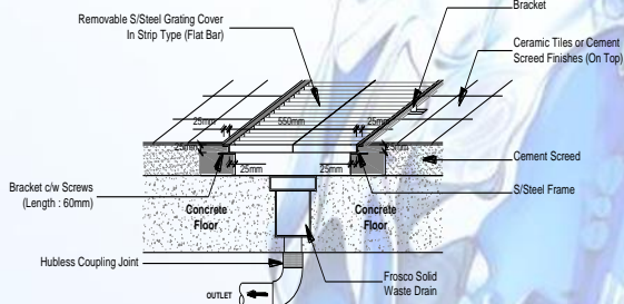
SECTION VIEW
