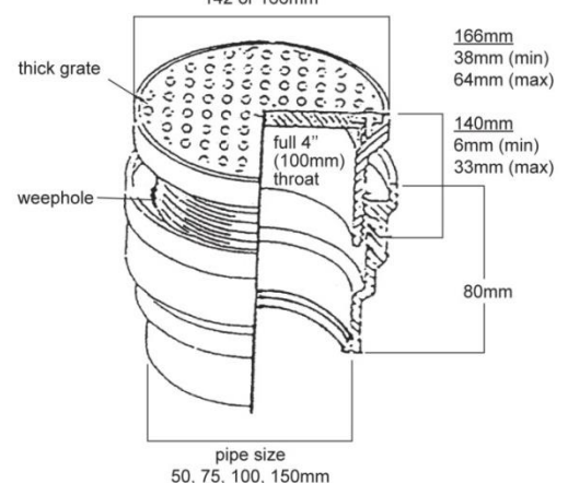
Perforated stainless steel sediment bucket
