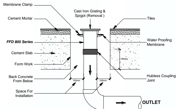
Detail A (FFD 800 Series)
