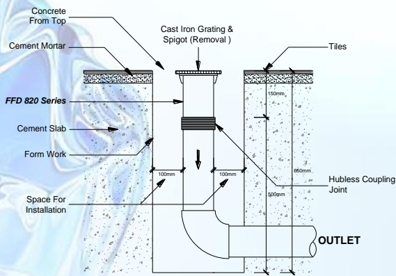
Detail B (FFD 820 Series)
